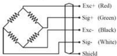
Wiring Diagram
